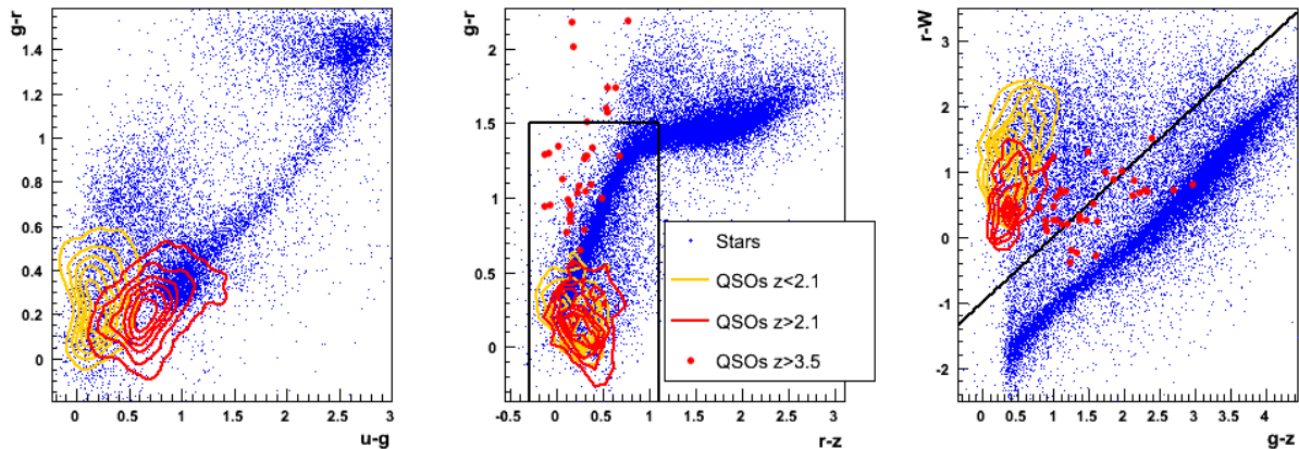
Figure 3.16: Colors in the optical ( ugriz ) or near-infrared (W is a linear combination of WISE W1 and W2 bands) of objects photometrically classified as stars (blue points) or spectroscopically classified as QSOs. Orange contours indicate the locus of tracer QSOs at z < 2.1 , red contours of Ly- \alpha QSOs at z > 2.1 , and red dots are for z > 3.5 QSOs. Left panel is based on SDSS photometry, middle and right panels on DECaLS-DR2. Black lines mark the boundaries of the selection regions described in the text. fig:colorsQSO
