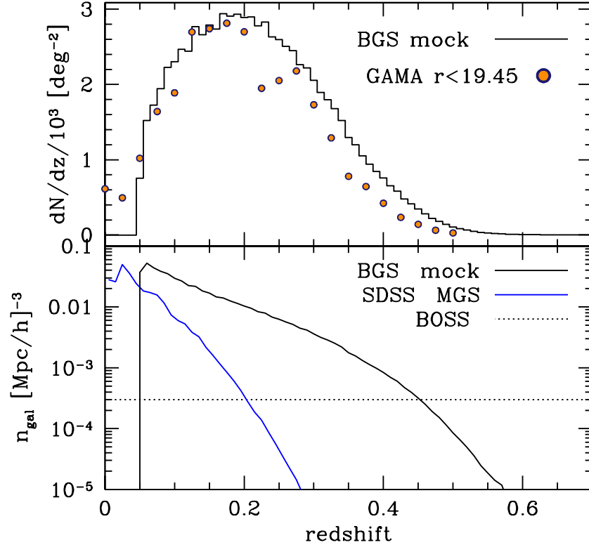
Figure 3.2: Upper panel: The redshift distribution of the mock BGS sample. The distribution peaks at z = 0.18 with a median redshift of z = 0.204 . Lower panel: The space density of BGS galaxies as a function of redshift. For comparison, the space density of the MGS is shown with the blue curve, and the approximate space density of the full BOSS LRG sample (LOWZ+CMASS) is shown with the dotted line. The space density of the BGS sample is larger than the MGS+BOSS samples up to z \sim 0.4 . fig:bgs_nz
