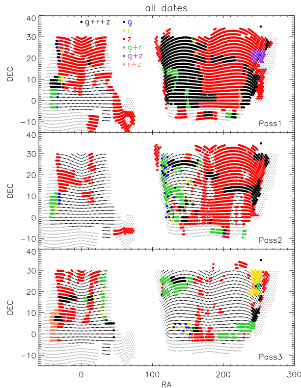
Figure 3.20: Left panel: Coverage map of the DECaLS survey through February 2016. The coverage in the g , r and z filters is indicated in each of the three passes. fig:DECCoverage
