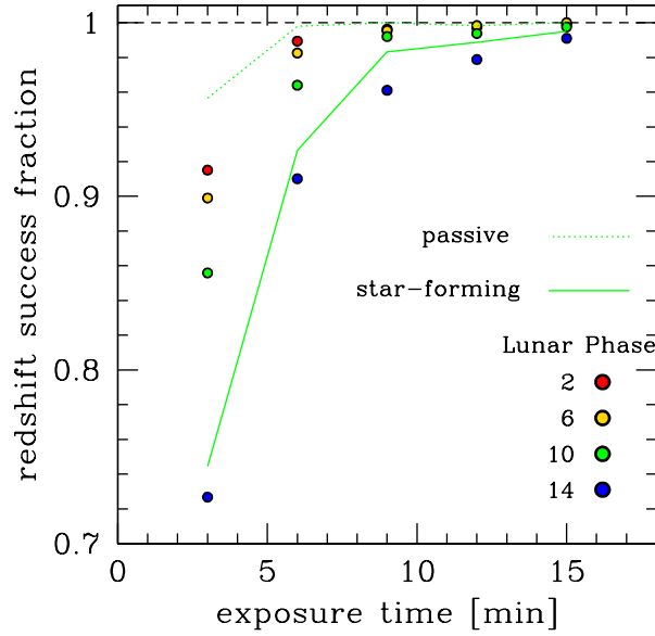
Figure 3.3: fig:bgs_redshift_efficiency The redshift success rate for BGS-like targets. Test targets are created by ‘observing’ MGS galaxies at twice the true redshift of the galaxies. Test spectra are created using desi_quicksim , incorporating a lunar model that incorporates the phase, zenith angle of the moon, zenith of the target, and the angle between the target and the moon. Results are shown as a function of exposure time and lunar phase. The green curves show the results for a 10-day lunar phase for passive and star-forming galaxies.
