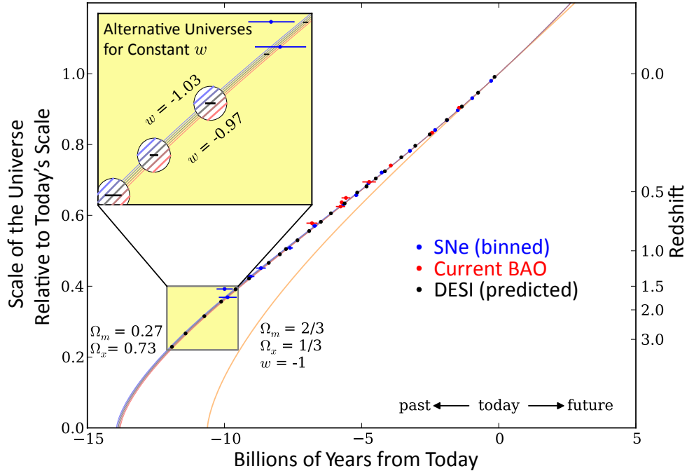
Figure 2.1: fig:rubin The expansion history of the Universe for different models of dark energy, holding the present-day Hubble constant fixed. The inset shows the spacing between five models with constant w ranging from -0.97 to -1.03 , showing the exquisite precision required to distinguish these. Overlaid are measurements of the distance-redshift relation, translated into errors on lookback time at each redshift. Measurements from current supernovae, binned in redshift, are shown in blue; current BAO measurements from BOSS DR9, WiggleZ, and 6dF are shown in red; projections for DESI are shown in black. DESI measurements have the ability to make very tight constraints on dark energy, although we caution that this figure shows variations in only one cosmological parameter. Full forecasts, such as those presented in § 2.4.3, must marginalize over other cosmological parameters such as \Omega_m and H_0 .
