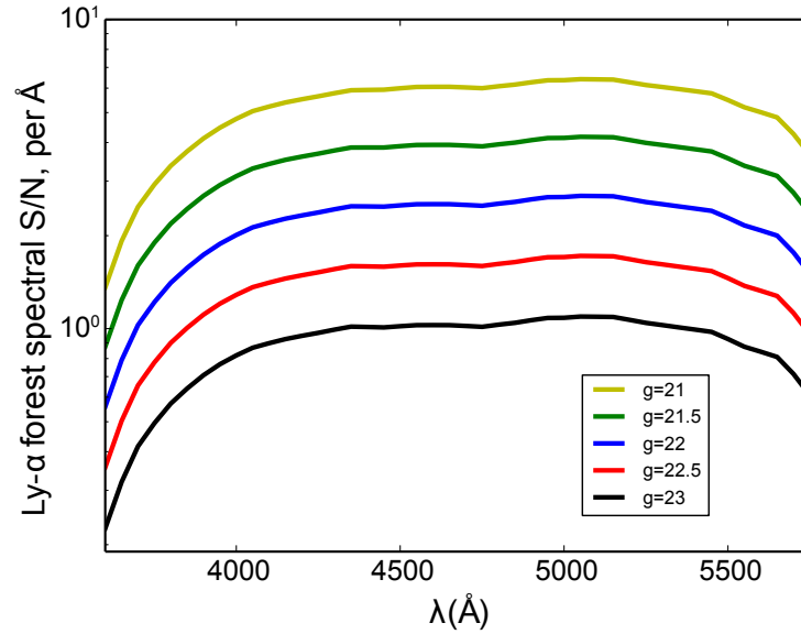
Figure 2.8: Signal-to-noise ratio per \text{\AA} used for DESI quasar spectra (detector noise, not absorption noise), for different g magnitudes, accounting for mean Ly- \alpha forest absorption. fig:qSN
