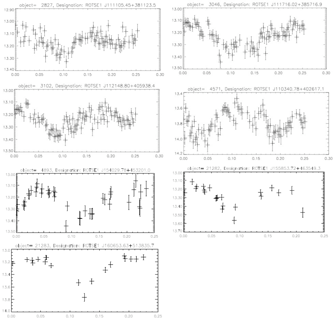
Figure 7: Single-night light curves for objects without a variable match and exhibiting irregular variations. Plotted errors are statistical + systematic. The x -axis represents the time of observation in days, while the y -axis represents the magnitude of an observation.
