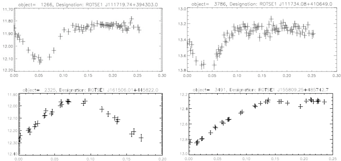
Figure 6: Single-night light curves for objects without a transient match. Lightcurves appear to be incomplete segments from regular variables. Errors are
