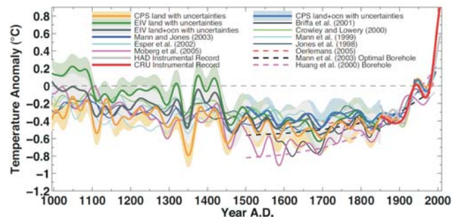
Various northern hemisphere temperature reconstructions. 40
