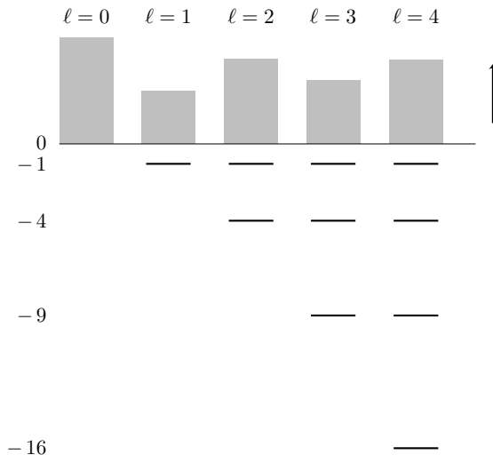
FIG. 1: Energy levels in reflectionless potentials.
