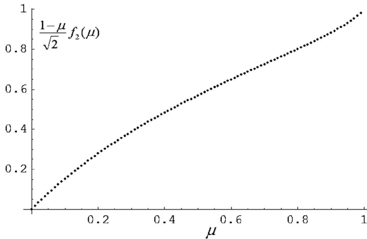
Fig. 5. Plot of [(1-\mu)/\sqrt{2}]f_2(\mu) . The plot shows that the function remains finite for all values of \mu .
