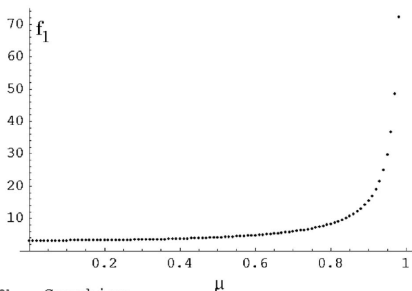
Fig. 2. The definition, evaluation, and plot of f_1(\mu) .
