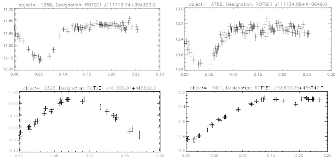
Figure 6: Single-night light curves for objects without a transient match. Lightcurves appear to be incomplete segments from regular variables. Errors are statistical + systematic. The x -axis represents the time of observation in days, while the
