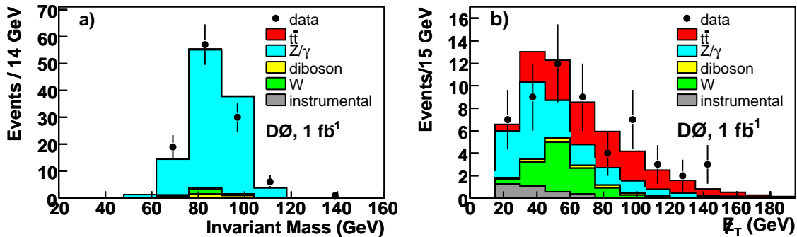
FIG. 1: Comparison of the expected distributions from backgrounds and t\bar{t} ( m_t = 170 GeV) in the \ell +track channels. (a) M_{\ell t} for the e +track channel without the requirement of the b -tag and with inverted E_T cuts. (b) E_T for the sum of both \ell +track channels, again without the b -tag requirement. We assume \sigma_{t\bar{t}} = 7.0 pb.
