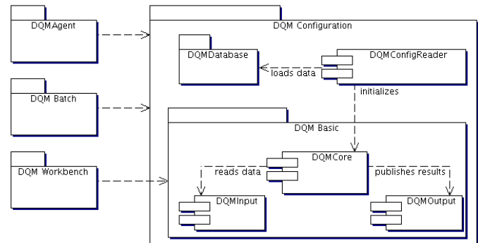
Fig. 5: Different environments to run DQMF.
