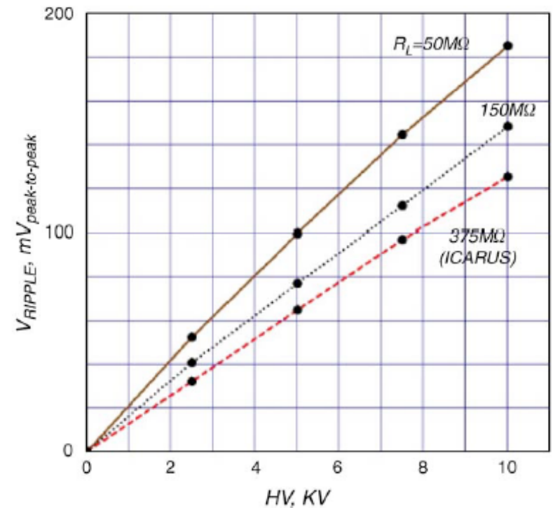
Fig. 41. Dependence of the voltage ripple (peak-to-peak) on the HV for different load resistors. (a) Solid line: R_L = 50 \text{ M}\Omega ; (b) dotted line: R_L = 150 \text{ M}\Omega ; (c) dashed line: R_L = 375 \text{ M}\Omega (T600 working conditions).
