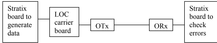
Fig. 6. Example of a LOC test link system. Here again the two Stratix blocks can be one or two boards. The LOC is an ASIC that integrates the serializer and the laser driver, maybe even the laser into one packaged chip. This ASIC is being developed based on a 0.25 \mu\text{m} silicon on sapphire CMOS technology for ATLAS LAr readout upgrade.
