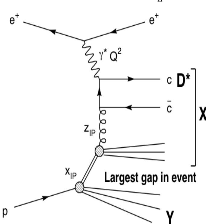
Representation of D^* diffractive production in the infinite-momentum frame description of DDIS
