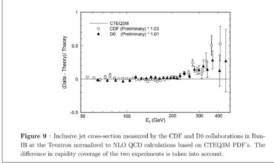
Figure 3: Comparison with the Tevatron jet data showing the differences at high E_T values.
