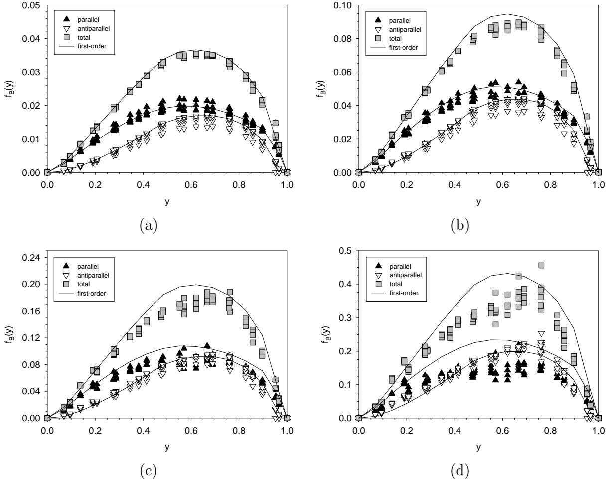
FIG. 2. The boson structure function f_B at various numerical resolutions for (a) \langle:\phi^2(0):\rangle = 0.1 , (b) \langle:\phi^2(0):\rangle = 0.25 , (c) \langle:\phi^2(0):\rangle = 0.5 , and (d) \langle:\phi^2(0):\rangle = 1.0 , with M = \mu , \Lambda^2 = 50\mu^2 , \mu_1^2 = 10\mu^2 , \mu_2^2 = 20\mu^2 , and \mu_3^2 = 30\mu^2 . The solid line is from first-order perturbation theory.
