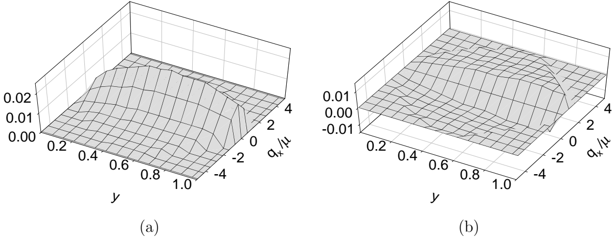
FIG. 6. The one-boson amplitude \phi_{\sigma s}^{(1,0,0,0)} , with (a) parallel ( s = \sigma ) and (b) antiparallel ( s = -\sigma ) bare helicity, as a function of longitudinal momentum fraction y and one transverse momentum component q_x in the q_y = 0 plane. The parameter values are K = 29 , N_{\perp} = 7 , M = \mu , \Lambda^2 = 50\mu^2 , \mu_1^2 = 10\mu^2 , \mu_2^2 = 20\mu^2 , \mu_3^2 = 30\mu^2 , and \langle:\phi^2(0): \rangle = 0.25 .
