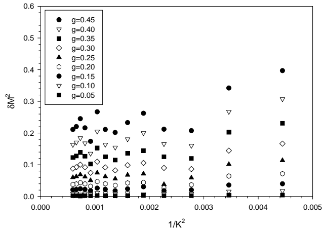
FIG. 7. The bare mass shift \delta M^2 as a function of the longitudinal resolution K for various bare couplings g , with N_{\perp} = 4 , M^2 = 0.001\mu^2 , \Lambda^2 = 50\mu^2 , \mu_1^2 = 10\mu^2 , \mu_2^2 = 20\mu^2 , and \mu_3^2 = 30\mu^2 .
