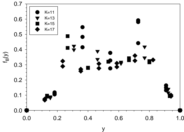
FIG. 1. The boson structure function f_B at various low to moderate numerical resolutions, with M = \mu , \langle :\phi^2(0): \rangle = 1.0 , \Lambda^2 = 50\mu^2 , \mu_1^2 = 10\mu^2 , \mu_2^2 = 20\mu^2 , and \mu_3^2 = 30\mu^2 . To compare with a structure function computed at higher resolutions, see Fig. 2(d).
