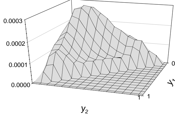
FIG. 5. The two-boson structure function \tilde{f}_{B\sigma} for K = 29 and N_{\perp} = 7 , with M = \mu , \langle:\phi^2(0): \rangle = 1 , \Lambda^2 = 50\mu^2 , \mu_1^2 = 10\mu^2 , \mu_2^2 = 20\mu^2 , and \mu_3^2 = 30\mu^2 .
